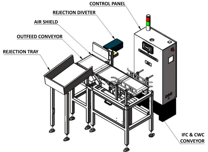
ISOMETRIC VIEW
